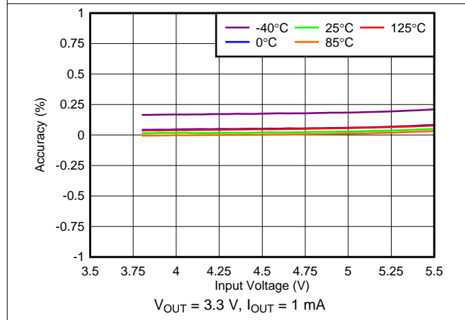
Figure 15. 3.3-V Regulation vs V_{IN} (Line Regulation)
