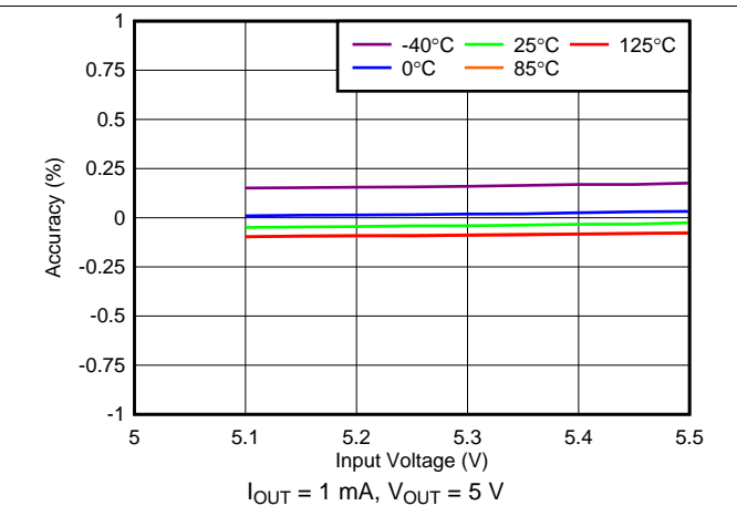
Figure 16. 5.0-V Accuracy vs V_{IN} (Line Regulation)
