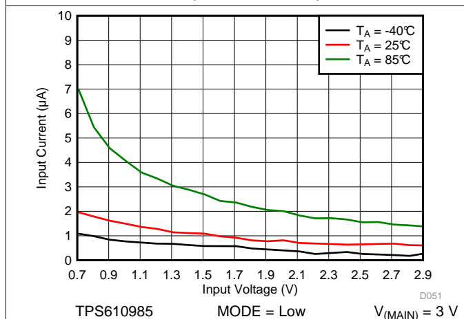
Figure 47. Input Current vs Input Voltage (Low Power Mode)
