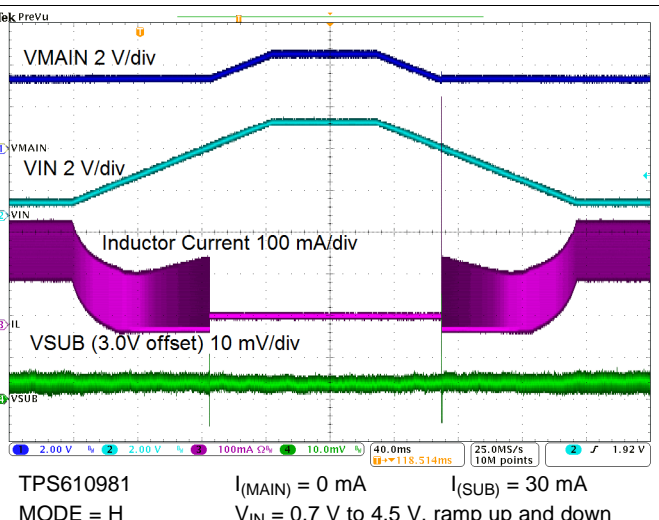
Figure 76. Line Regulation
