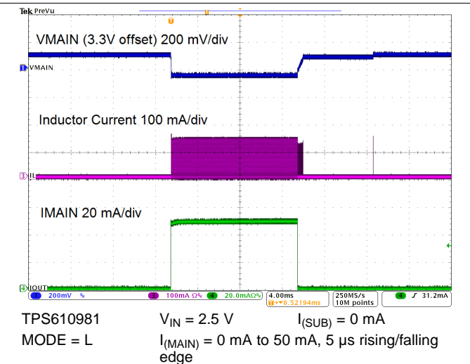
Figure 68. Load Transient Response
