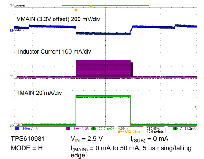
Figure 69. Load Transient Response
