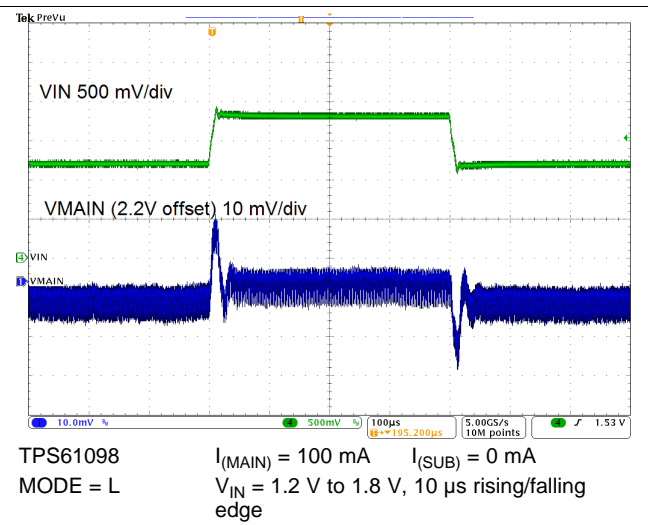
Figure 83. Line Transient Response
