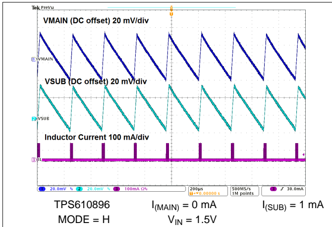
Figure 65. Switching Waveforms
