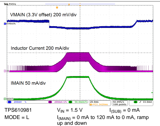
Figure 74. Load Regulation
