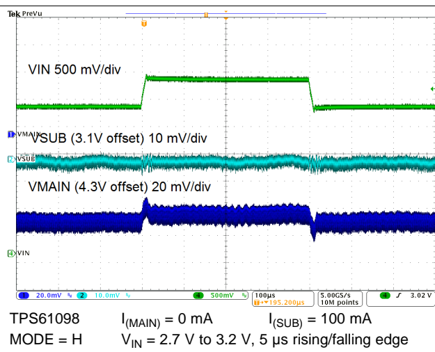
Figure 87. Line Transient Response
