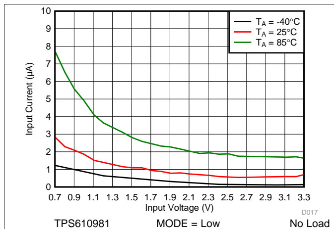
Figure 43. Input Current vs Input Voltage (Low Power Mode)
