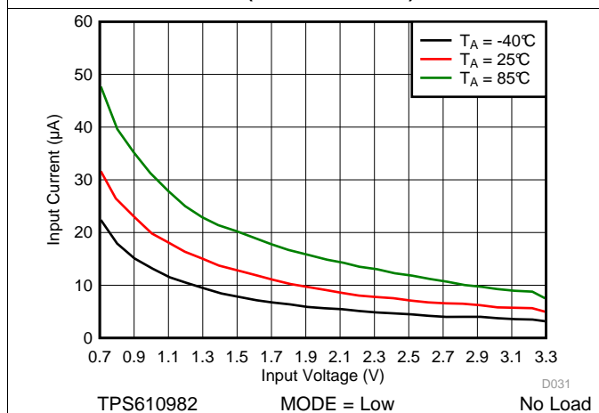
Figure 45. No Load Input Current vs Input Voltage (Low Power Mode)
