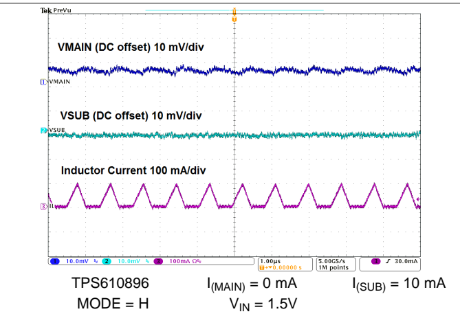
Figure 66. Switching Waveforms
