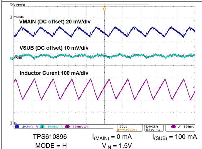
Figure 67. Switching Waveforms
