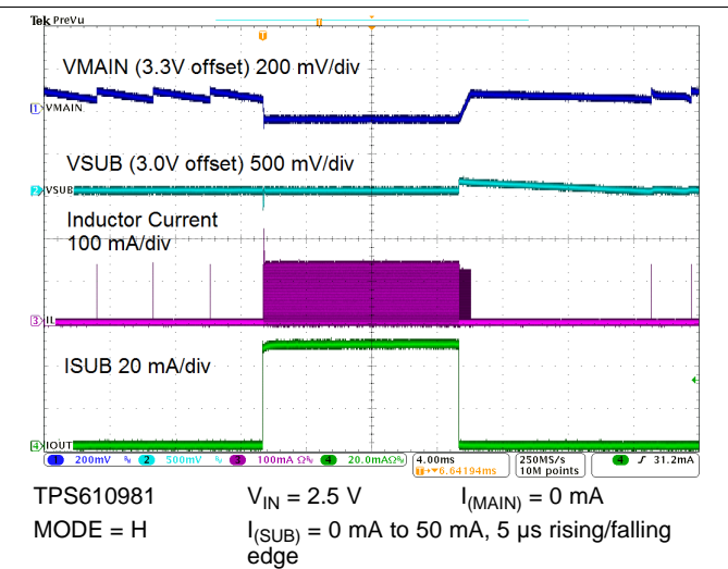
Figure 70. LDO Load Transient Response
