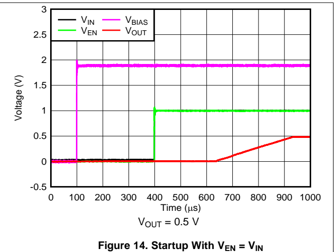
Figure 14. Startup With V_{EN} = V_{IN}
