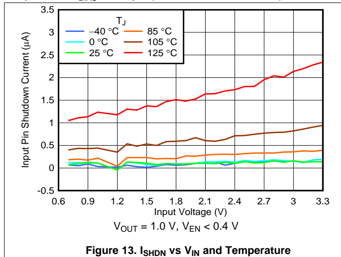
Figure 13. I_{SHDN} vs V_{IN} and Temperature
