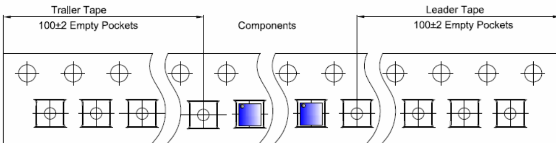
DFNWB2x2-6L Tape Leader and Trailer
