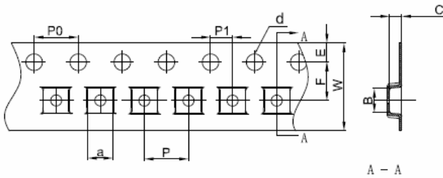
DFNWB2x2-6L Embossed Carrier Tape
