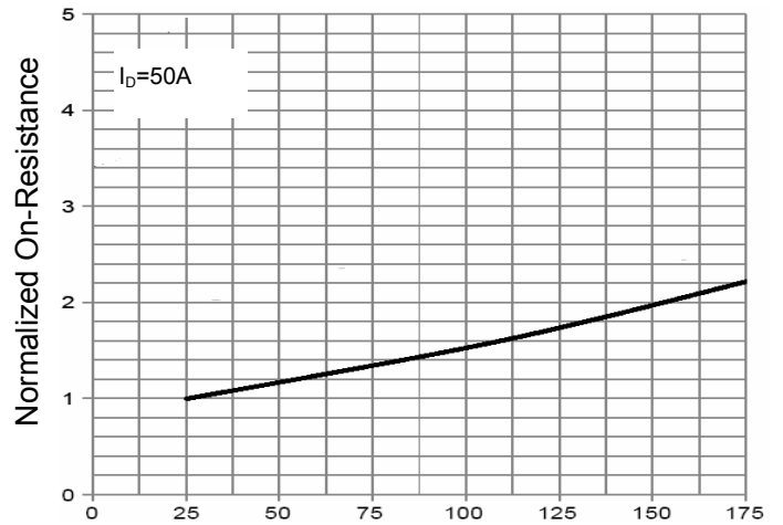
T J -Junction Temperature(°C) Figure 10 R ds(on) -Junction Temperature
