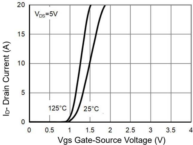
Figure 7 Transfer Characteristics
