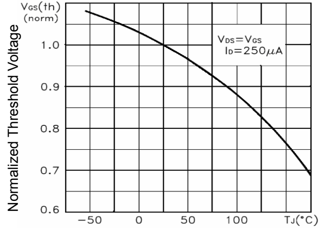
T_J -Junction Temperature( ^\circ C ) Figure 14 V_{GS(th)} VS Junction Temperature
