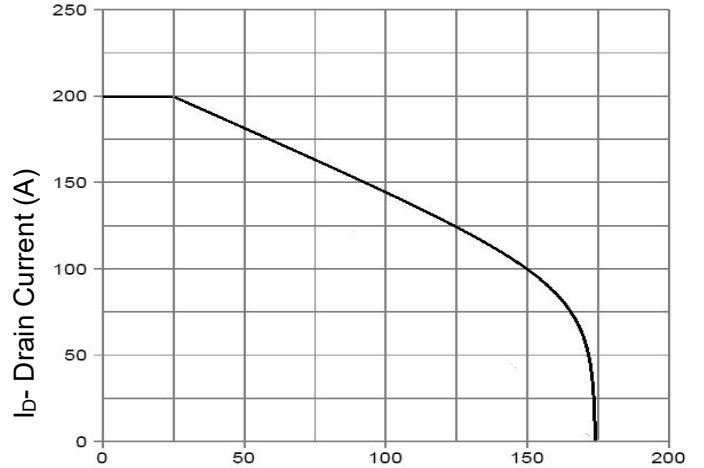
T A -Junction Temperature (°C) Figure 10 Current De-rating
