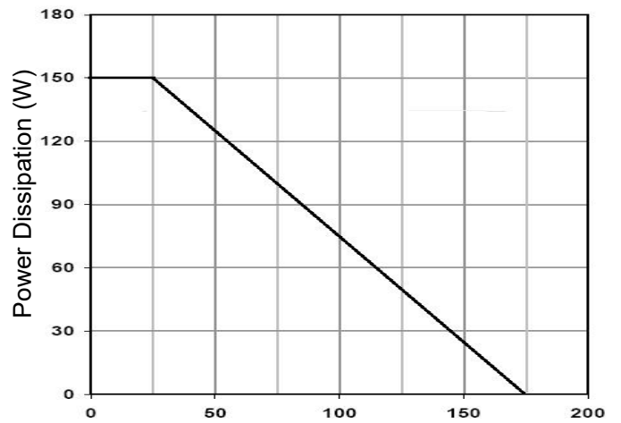
T_A -Junction Temperature( ^{\circ}C ) Figure 9 Power De-rating
