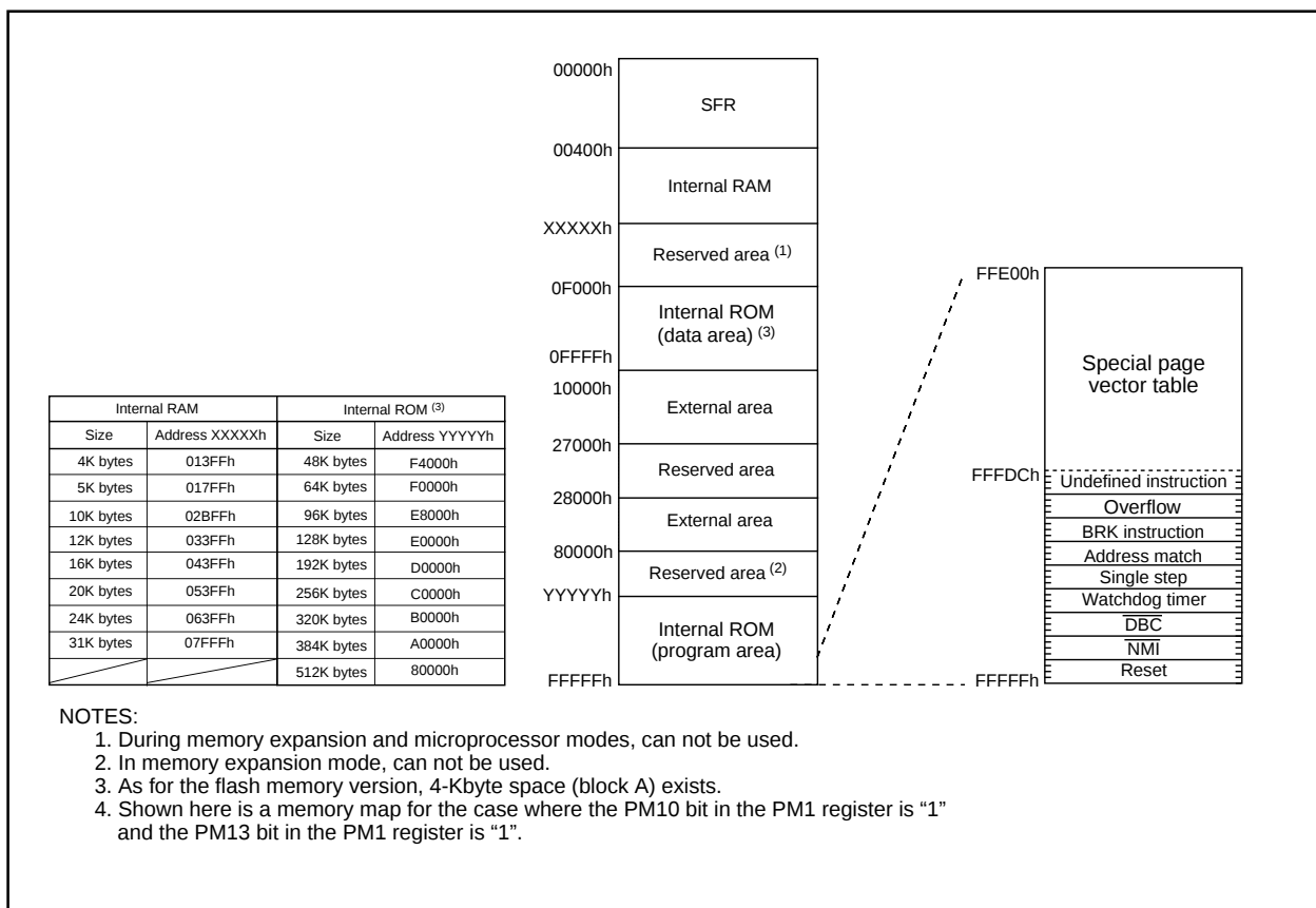
Figure 3.1 Memory Map
