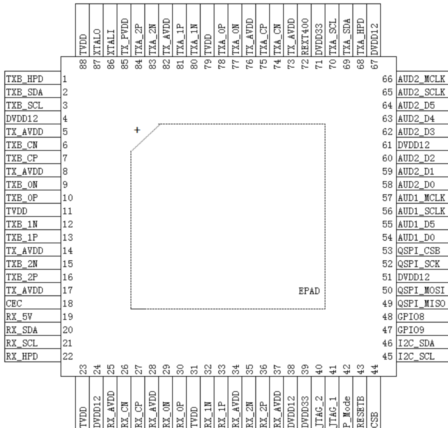
GSV6502 QFN88 Pin Diagram
